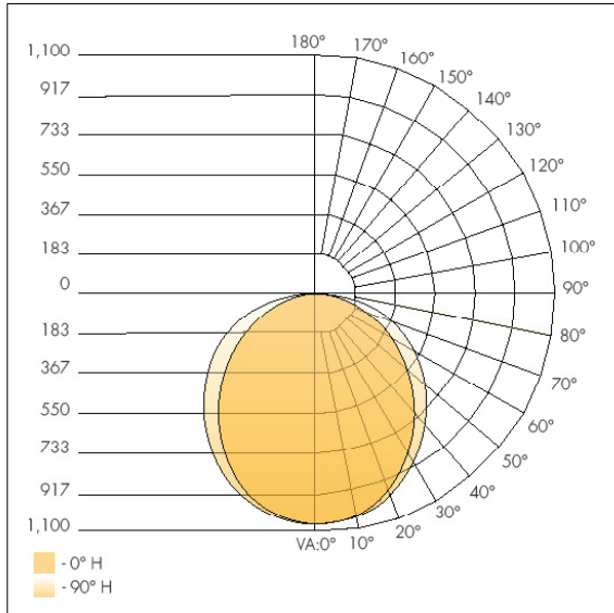
Polar Graph- 2x4 35W 4000K
